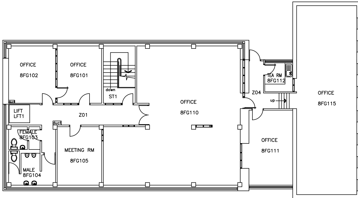
FIRST FLOOR
